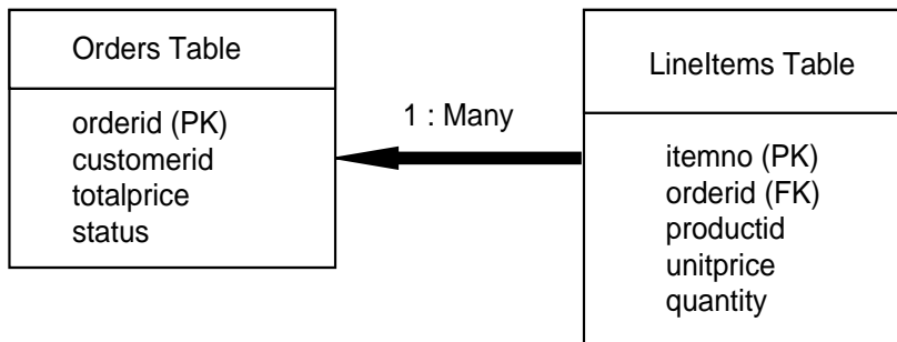
Figure 15 One-to-Many Relationship: Order and Line Items
