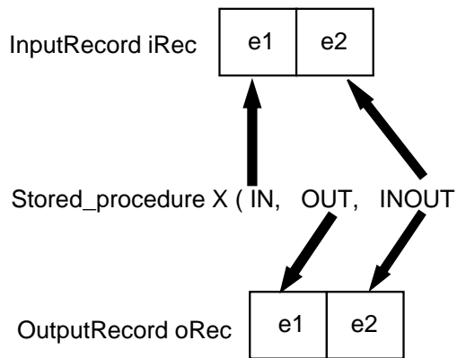
Figure 37 Mapping Stored Procedure Parameters to CCI Record Elements
