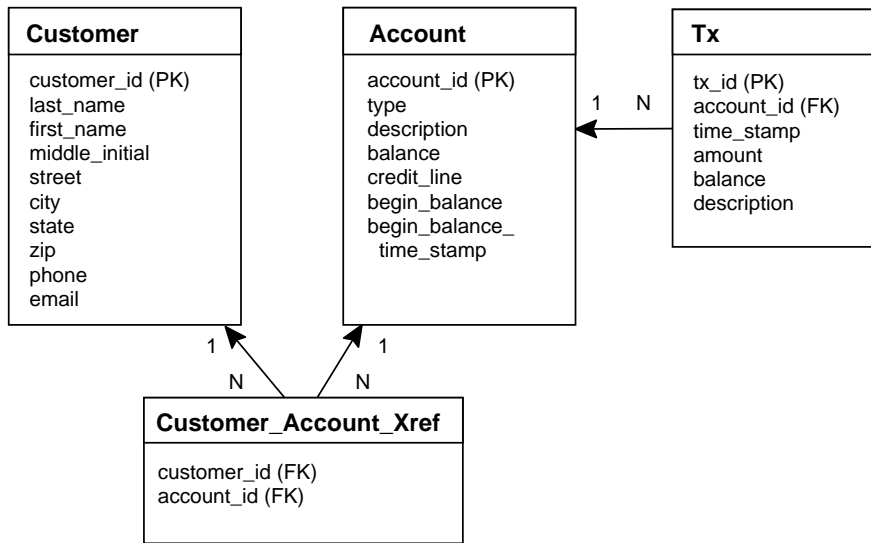
Figure 40 Database Tables in the Duke’s Bank Application
