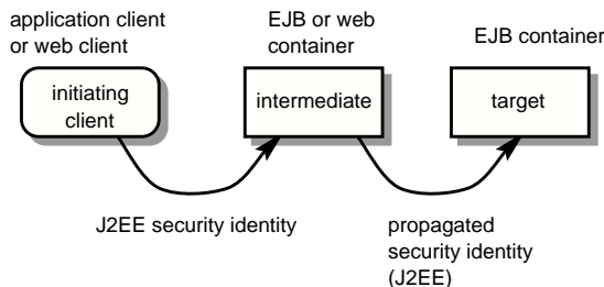
Figure 35 Security Identity Propagation
