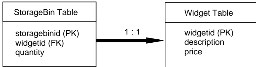
Figure 14 One-to-One Table Relationship
