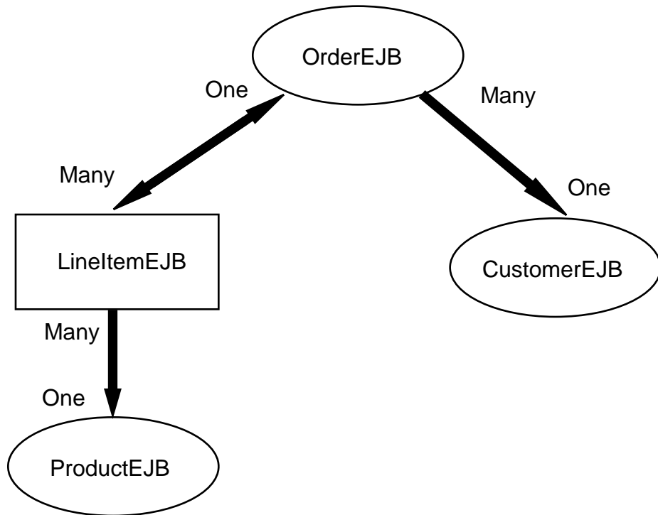
Figure 8 A High-Level View of an Abstract Schema
