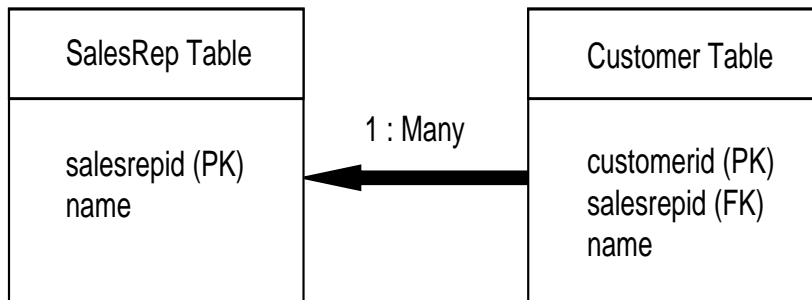
Figure 16 One-to-Many Relationship: Sales Representative and Customers
