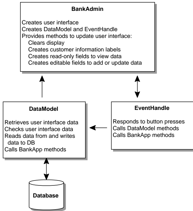
Figure 42 Relationships among Classes
