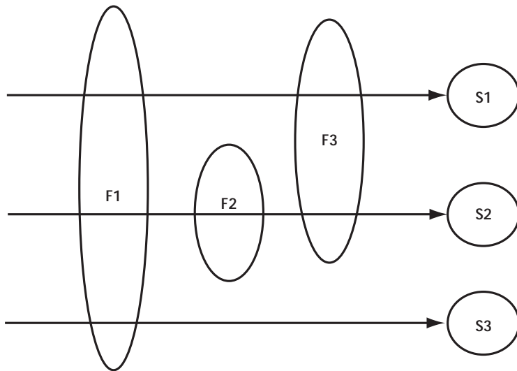
Figure 26 Filter to Servlet Mapping
