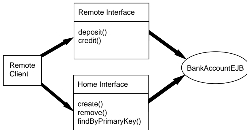
Figure 9 Interfaces for an Enterprise Bean With Remote Access
