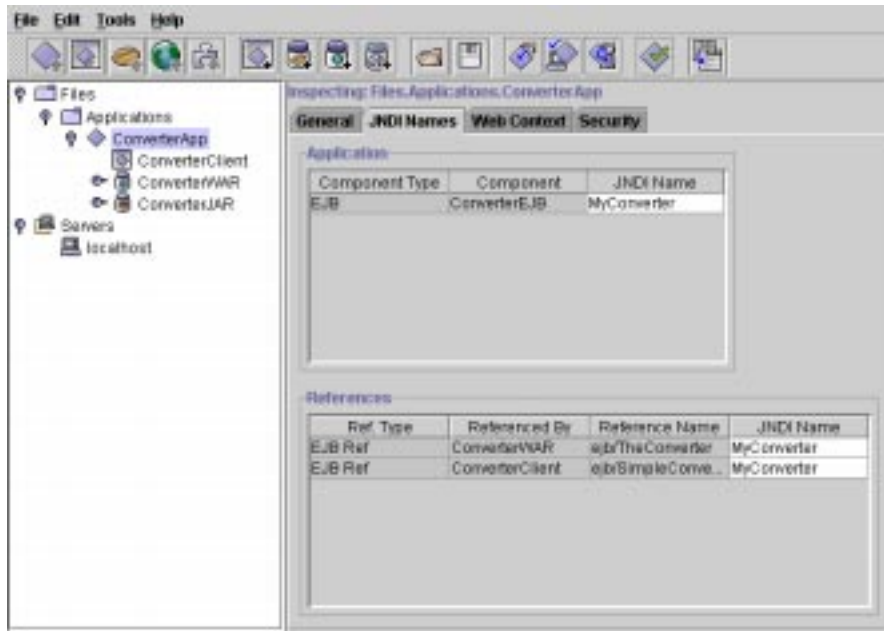
Figure 6 ConverterApp JNDI Names
