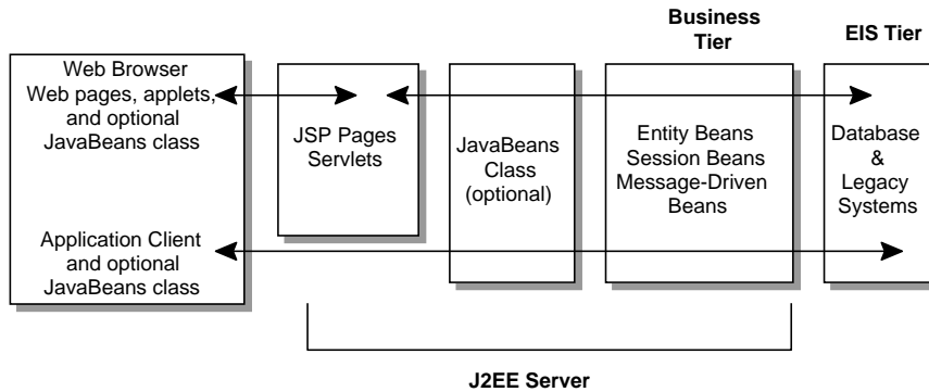
Figure 4 Business and EIS Tiers
