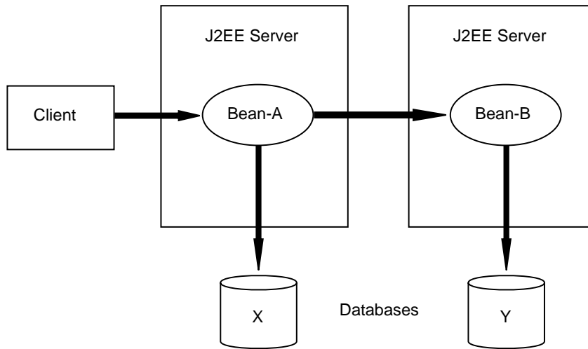
Figure 34 Updating Multiple Databases Across J2EE Servers
