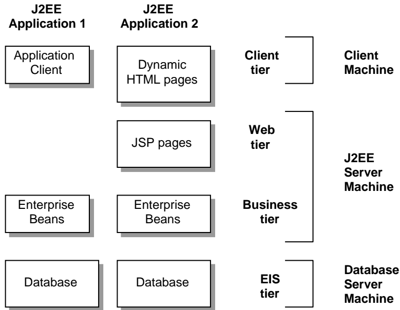
Figure 1 Multitiered Applications
