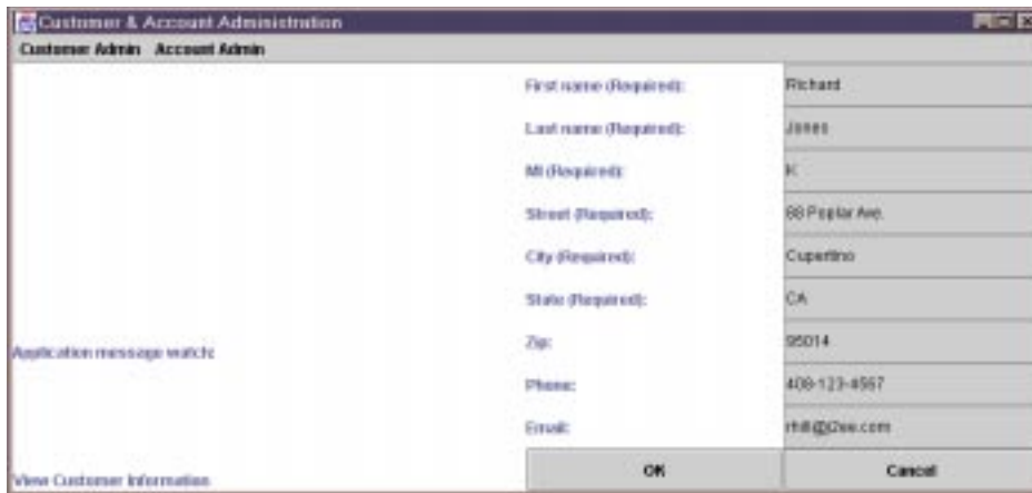
Figure 41 Application Client
