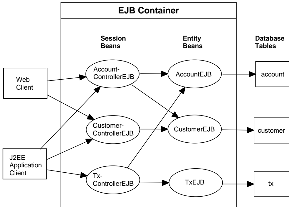
Figure 39 Enterprise Beans in the Duke's Bank Application
