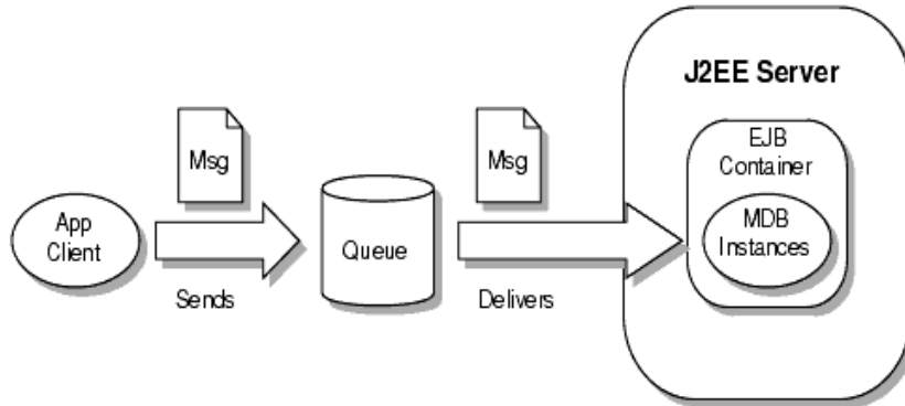
Figure 19 The SimpleMessageApp Application
