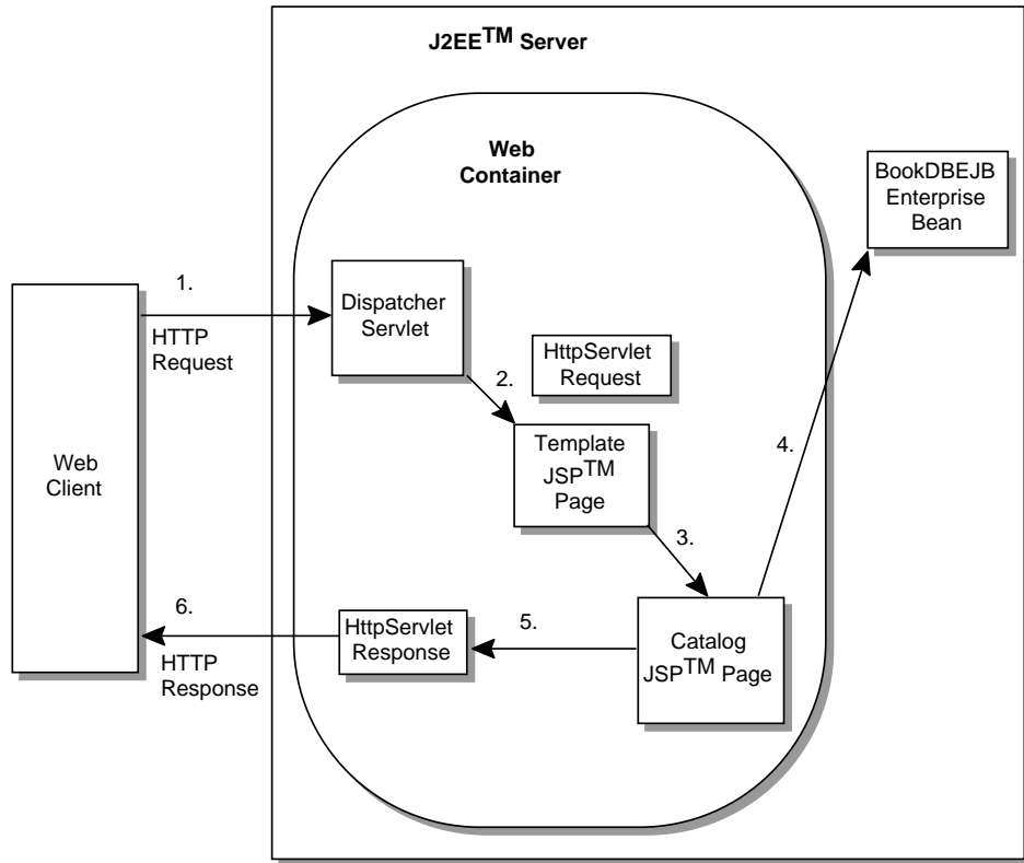
Figure 31 Request Flow Through Duke's Bookstore Components
