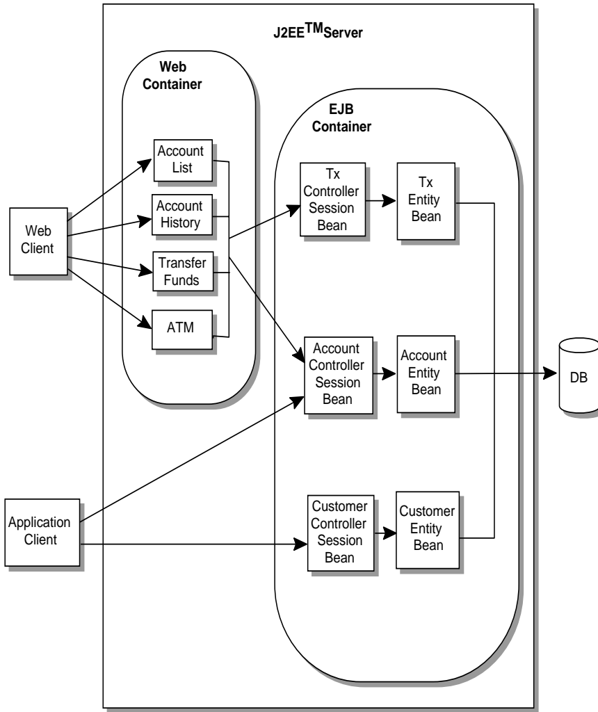
Figure 38 Duke's Bank Application
