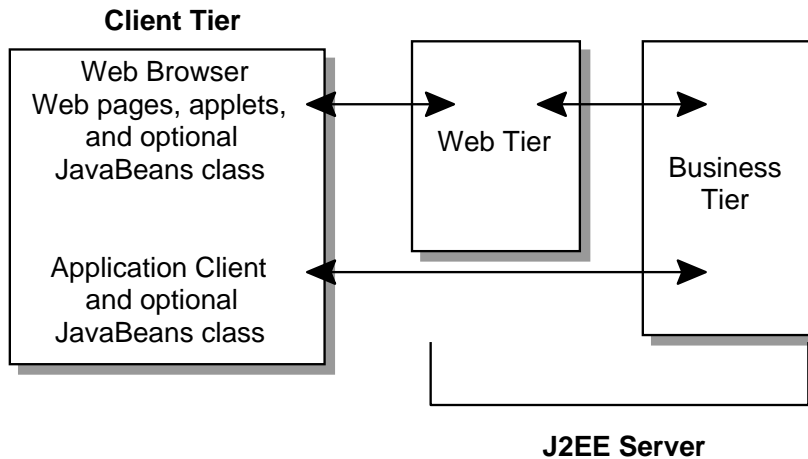
Figure 2 Server Communications
