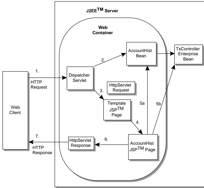
Figure 44 Web Component Interaction
