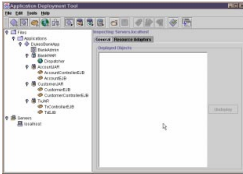
Figure 45 Duke's Bank Application Archives and Components
