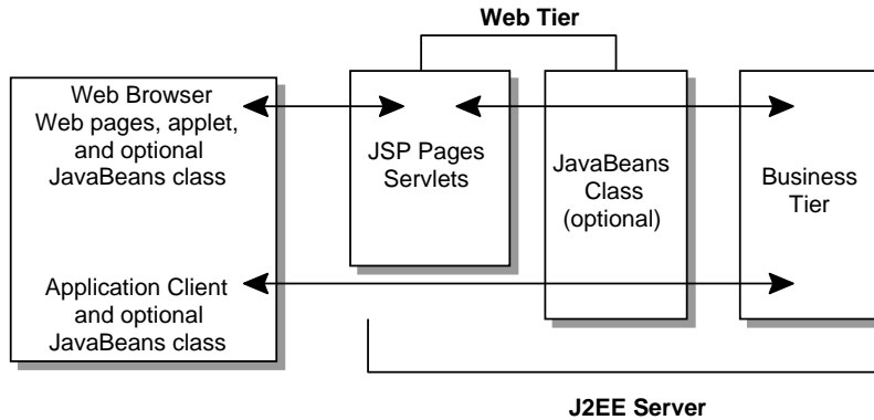
Figure 3 Web Tier and J2EE Application
