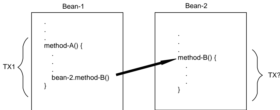
Figure 32 Transaction Scope
